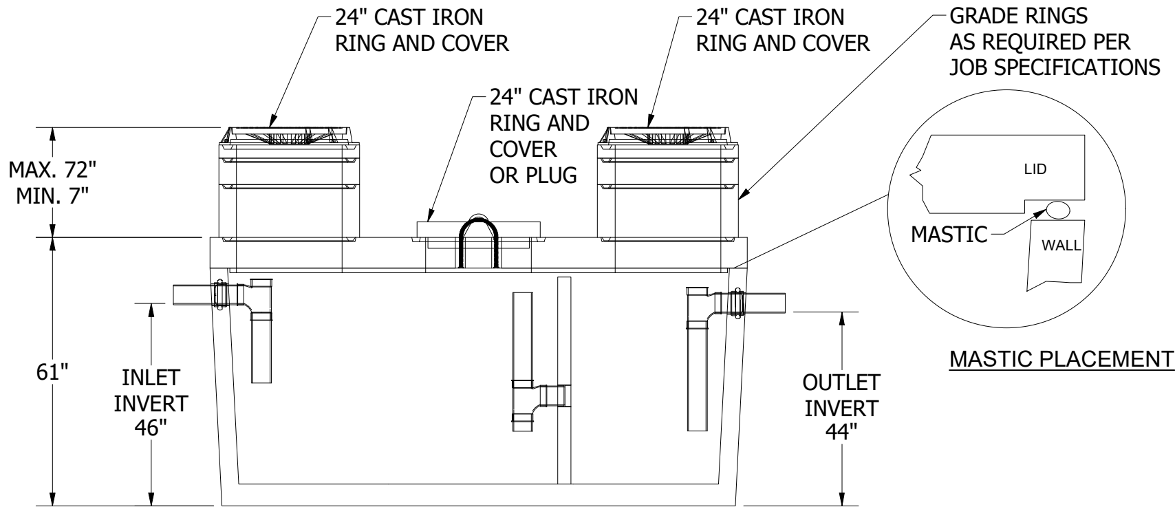
ELEVATIONS AND PROFILE VIEW
