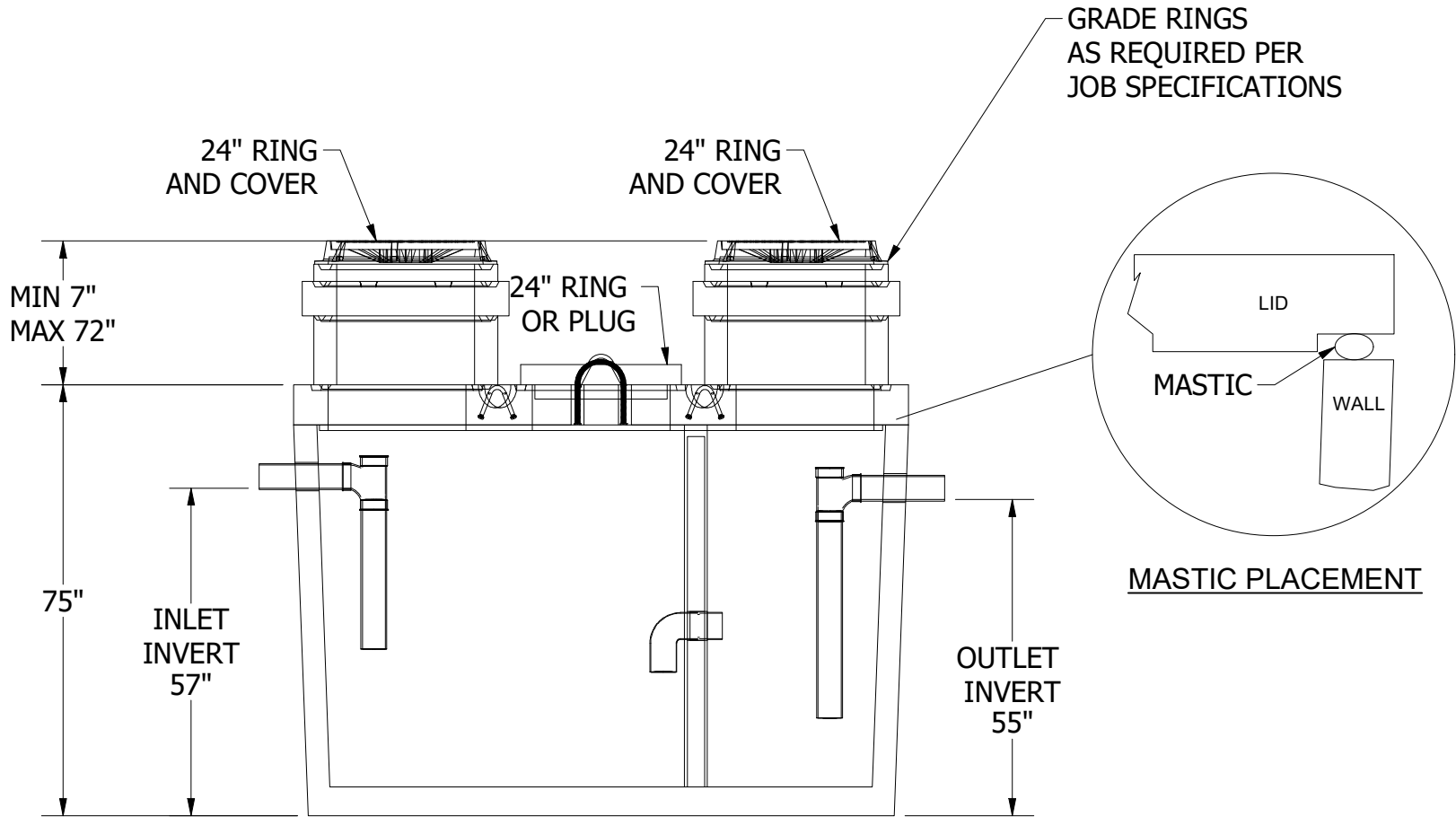
ELEVATIONS AND CROSS SECTIONAL
