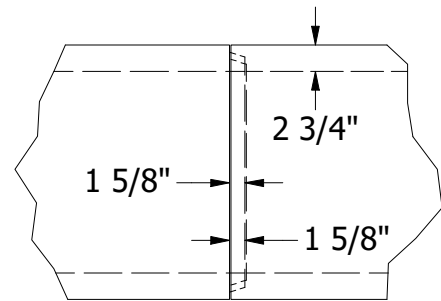
TONGUE AND GROOVE JOINT DETAIL
