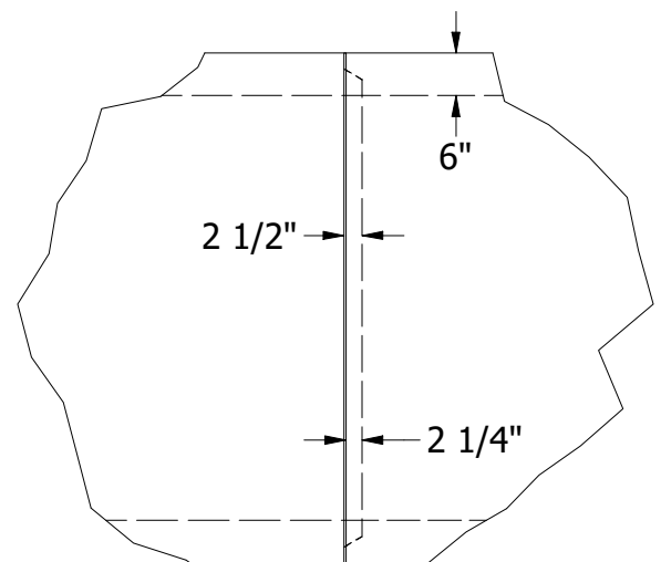
TOUNGE AND GROOVE JOINT DETAIL
