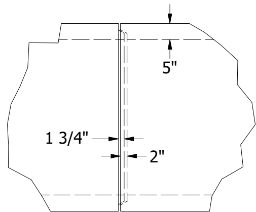
TONGUE AND GROOVE JOINT DETAIL
