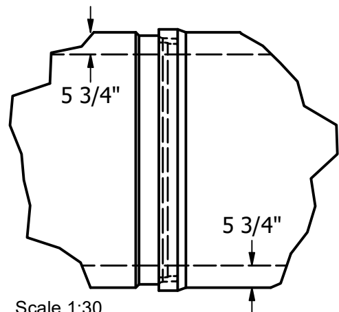
RUBBER GASKET JOINT DETAIL
