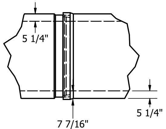
RUBBER GASKET JOINT DETAIL
