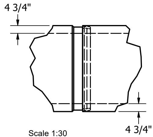
RUBBER GASKET JOINT DETAIL
