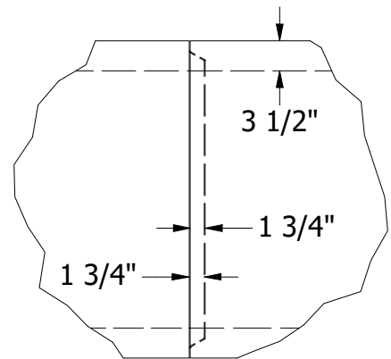
TONGUE AND GROOVE JOINT DETAIL
