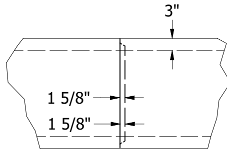
TOUNGE AND GROOVE JOINT DETAIL
