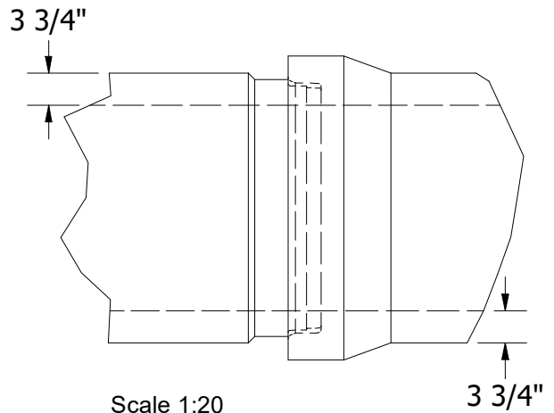
RUBBER GASKET JOINT DETAIL
