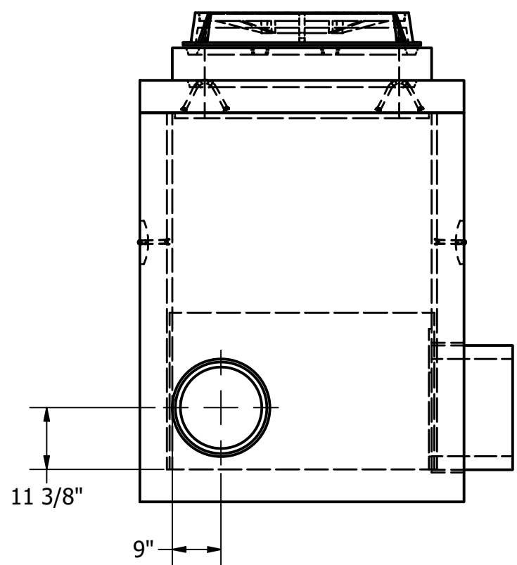
END VIEW
